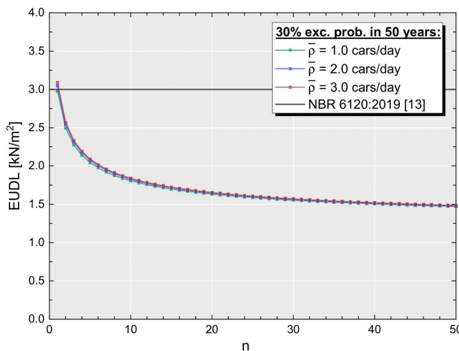
Figure 12. Sensitivity of the 50-year maximum EUDL with respect to temporal parameters.
