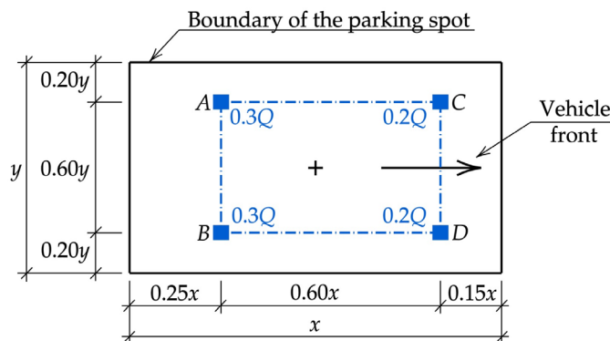
Figure 2. Vehicle placement in parking spot and load distribution.
