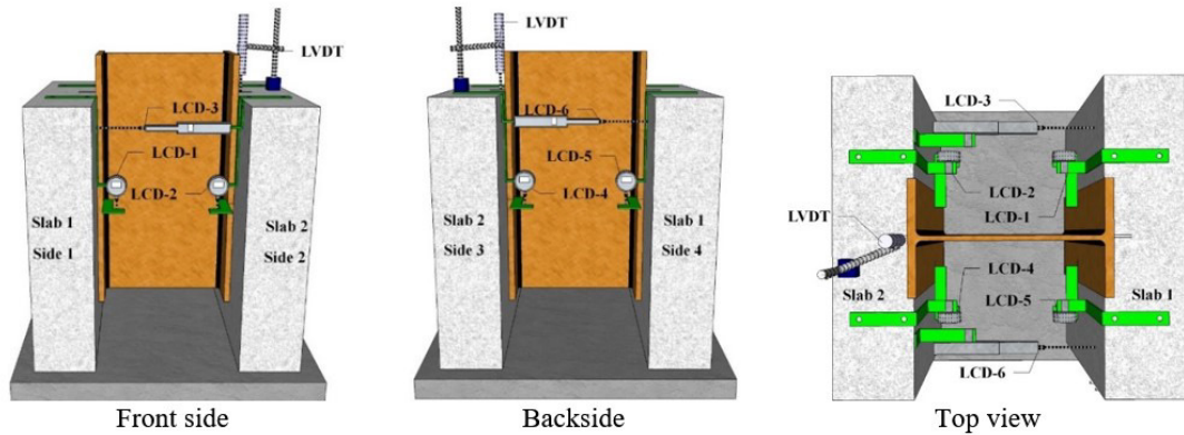
Figure 5. Instrumentation setup
