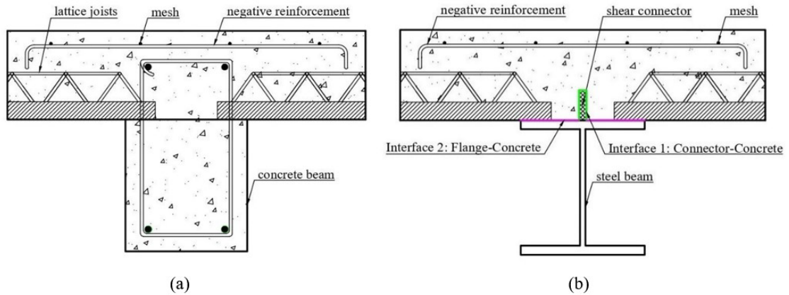
Figure 2. (a) Conventional floor system with lattice joists slab. (b) New proposed system for composite beam – Interfaces
