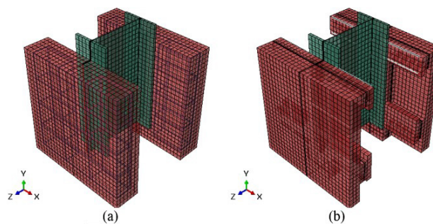
Figure 13. (a) MAC – FE model; (b) TREL – FE model
