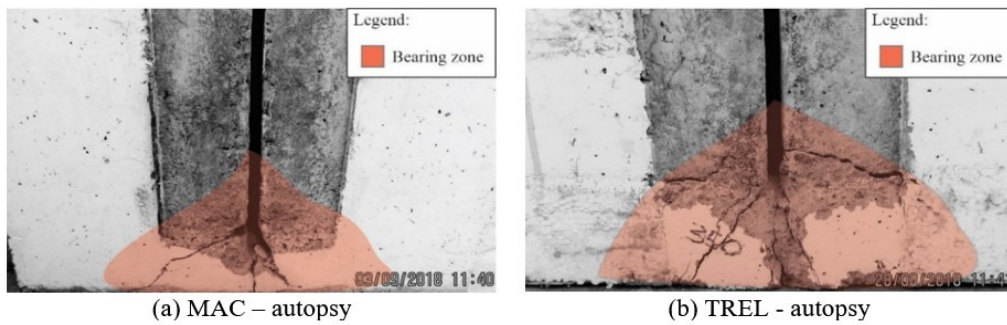
Figure 16. Failure modes of the specimens: (a) MAC; (b) TREL
