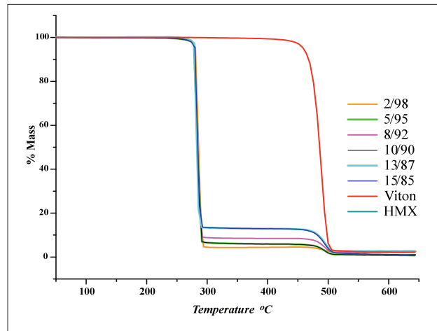
Figure 3: TG Curves of the system HMX/Viton sample in atmosphere of N 2
