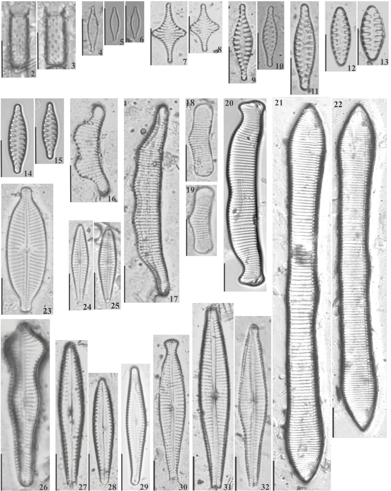
Figures 2-32. Holocene diatoms from Xingu river, Brazil. Diatoms of Xingu core. 2-3. Aulacoseira cf. crassipunctata Krammer. 4-6. Rimoneis sp. 7-8. Staurosira sp. 9-10. Staurosirella acidophila Almeida, Wetzel, Morales, Ector & Bicudo. 11. Staurosirella cf. acutirostrata (Metzeltin & Lange-Bertalot) Almeida & Wetzel. 12-13. Staurosirella dubia (Grunow) E.A.Morales & K.M.Manoylov. 14-15. Staurosirella subcapitata (Frenguelli) Morales. 16. Eunotia camelus Ehrenberg. 17. Eunotia longicamelus Costa, Wetzel, Lange-Bertalot, Ector & Bicudo. 18-19. Eunotia rabenhorstii var. monodon Cleve & Grunow. 20. Eunotia superbidens Lange-Bertalot. 21-22. Eunotia sp. 23. Placoneis exigua (W. Gregory) Mereschkovsky. 24-25. Gomphonema auritum Braun ex Kützing. 26. Gomphonema acuminatum Ehrenberg. 27-28. Gomphonema brasiliensoides Metzeltin, Lange-Bertalot & Garcia-Rodríguez. 29. Gomphonema curvipedatum Kobayasi ex Osada. 30. Gomphonema pseudosphaerophorum Kobayasi. 31-32. Gomphonema sp. Scale bars = 10 µm.
