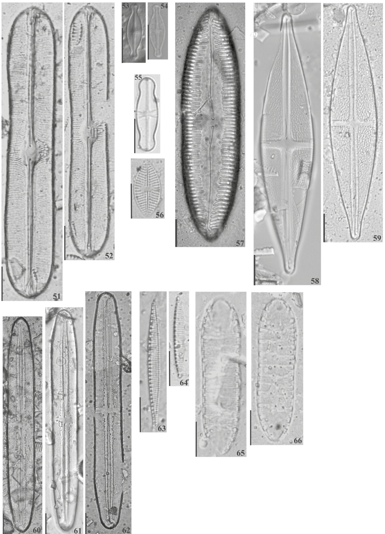
Figures 51-66. Holocene diatoms from Xingu river, Brazil. 51-52. Sellaphora renata Metzeltin & Lange-Bertalot. 53-54. Sellaphora sassiana (D. Metzeltin & H. Lange-Bertalot) C.E. Wetzel. 55. Sellaphora ventraloconfusa (Lange-Bertalot) Metzeltin & Lange-Bertalot. 56. Lacuneolimna novagallia Tudesque & Le Cohu 57. Pinnularia cf. liyanlingae Metzeltin & Lange-Bertalot. 58-59. Stauroneis sp. 60-62. Stauroneis sp.1. 63-64. Nitzschia pusilluhasta E.A.Lehmkuhl & C.E.M.Bicudo. 65-66. Surirella sp. Scale bars = 10 \mu m.
