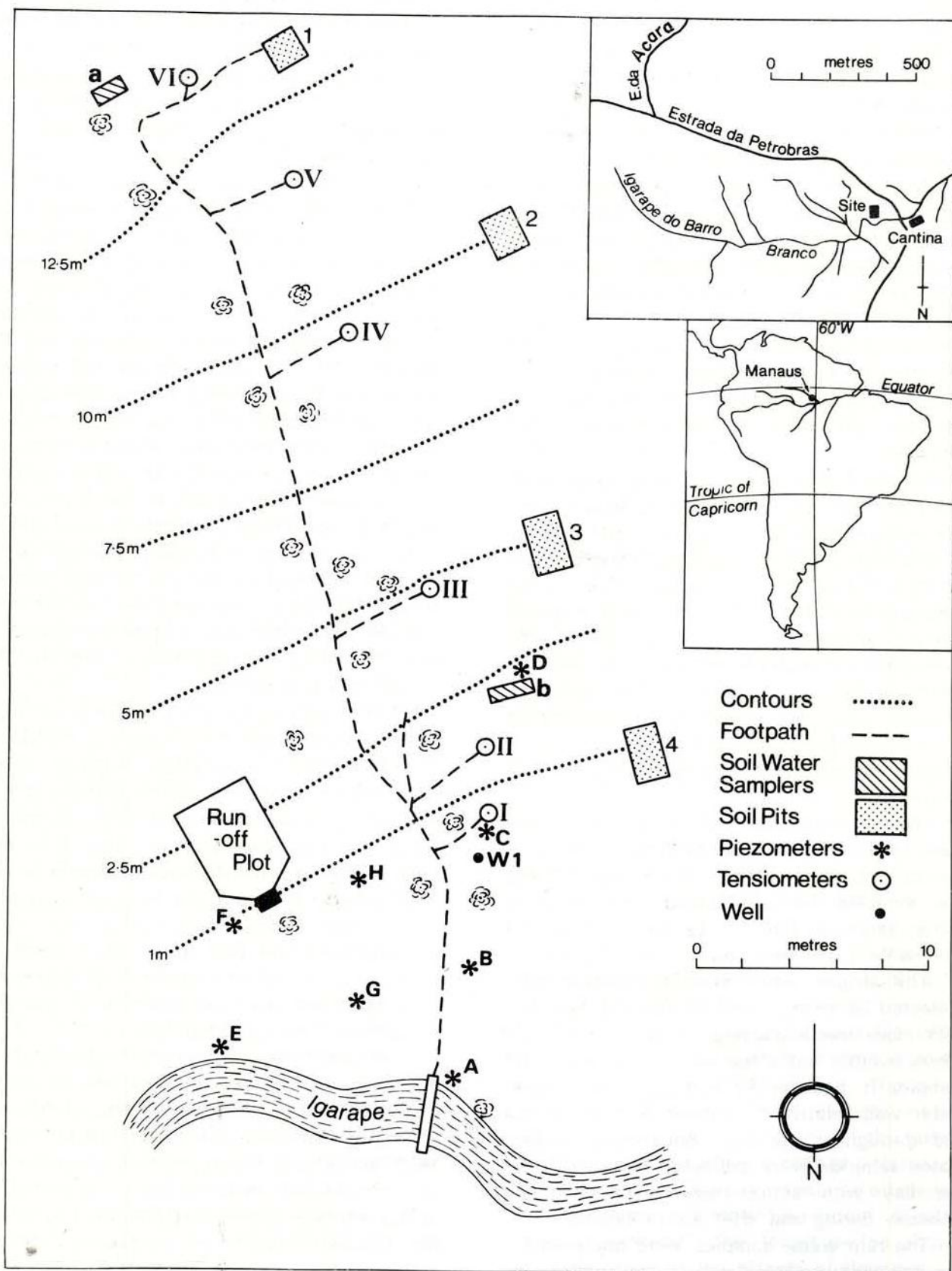
Fig. 2 — Instrumentation of hillslope.
