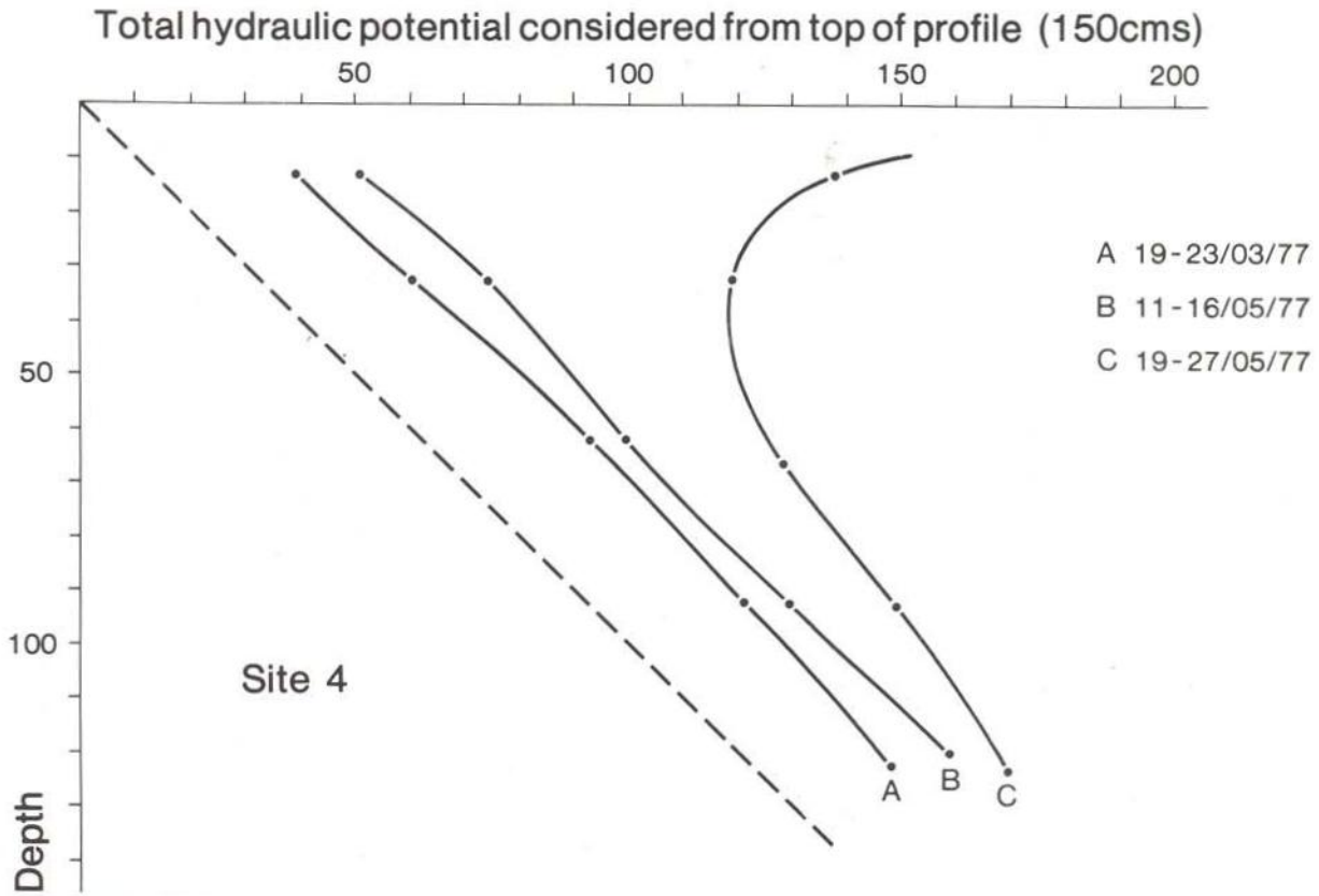
Fig. 5 — Distribution of total hydraulic potential with reference to top of profile.
