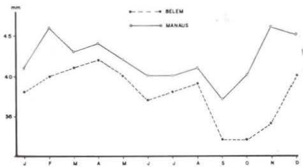
Fig. 4 — Monthly values of precipitable water ( W_p ) for 1972.
