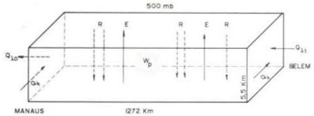
Fig. 2 — Model utilized for characterization of the components of the atmospheric branch of the hidrologic cycle.
