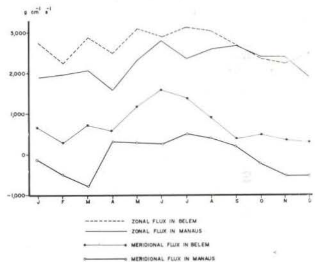
Fig. 5 — Zonal and meridional fluxes obtained in 1972 for Belem and Manaus.
