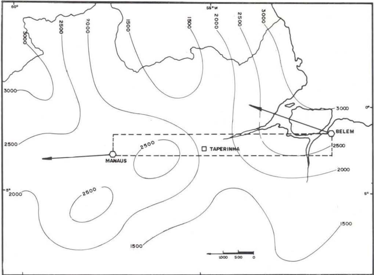
Fig. 3 — Total precipitation (in mm) in 1972. The arrows indicate the total vapor flux over Belem and Manaus (1cm = 500g/cm.s).
