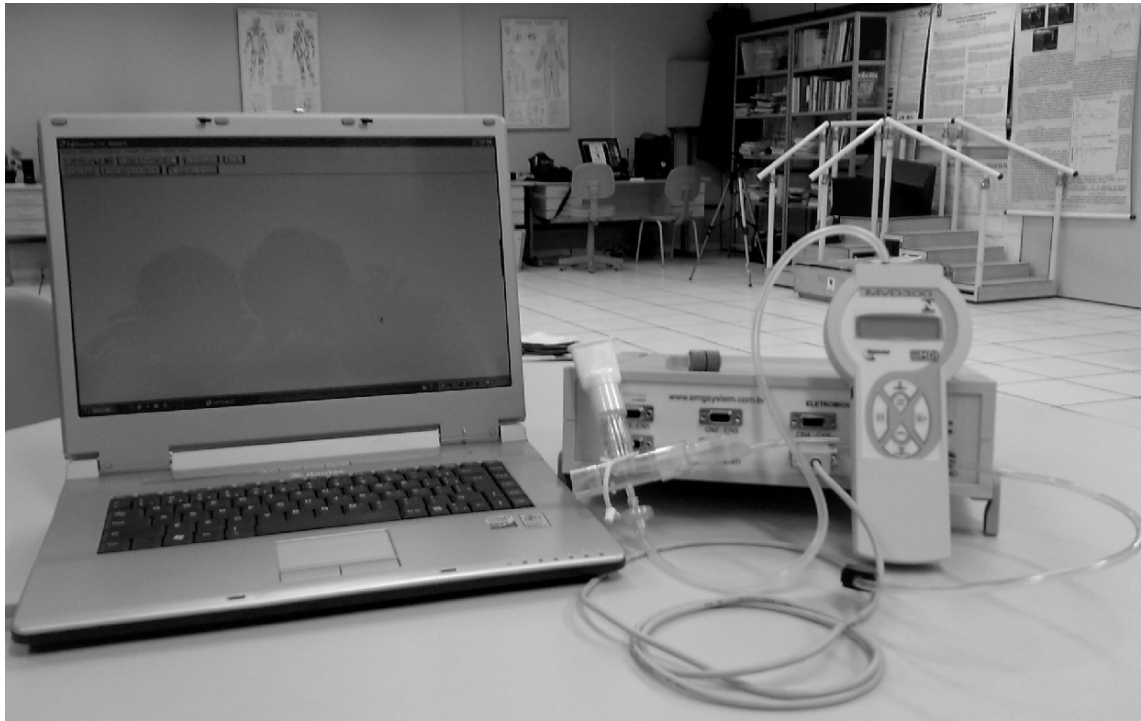
Fig. 1 – Computer, signal conditioner and portable digital monometer.
