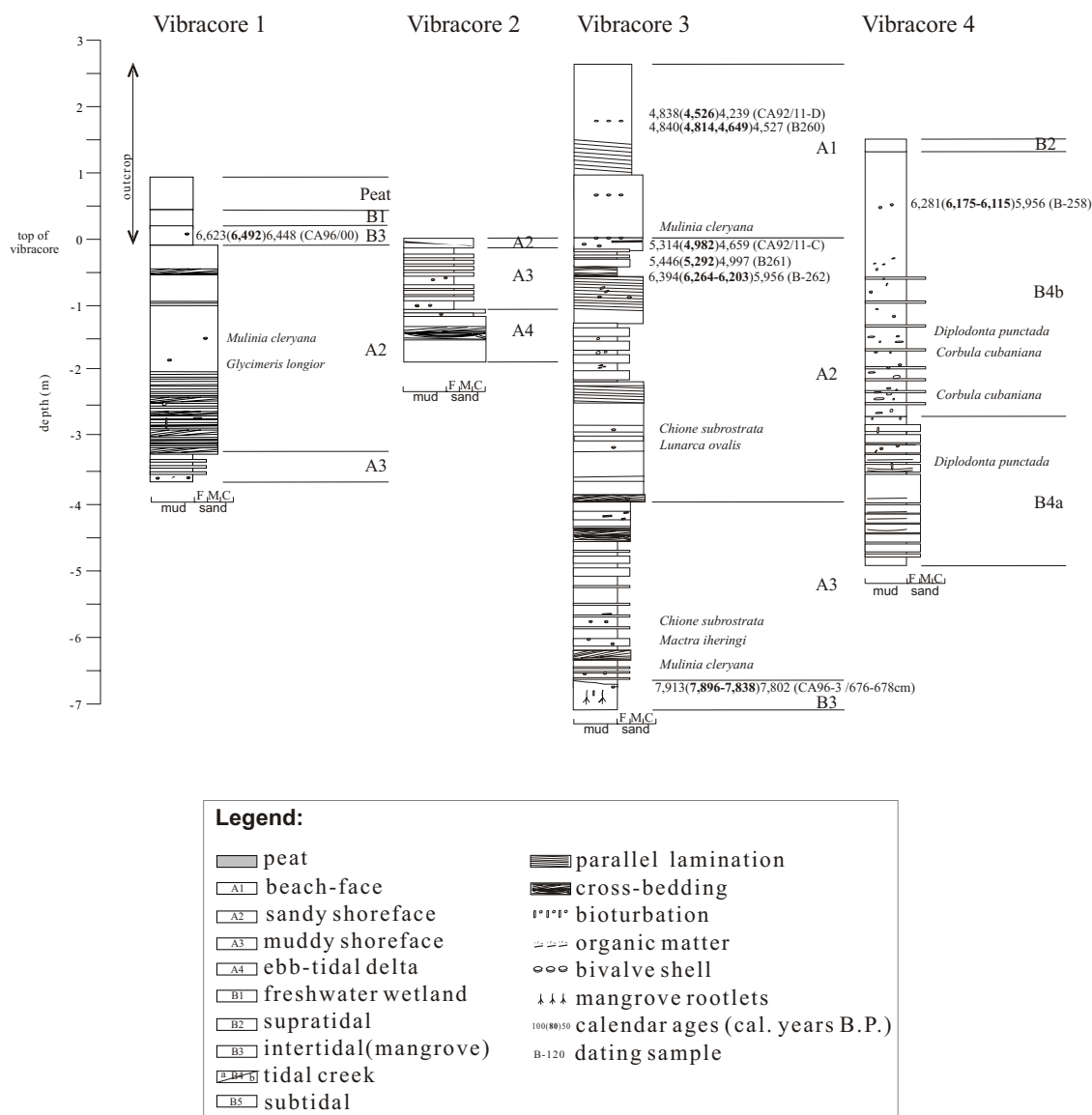
Fig. 6 – Sedimentary facies of vibracores 1, 2, 3 and 4.
