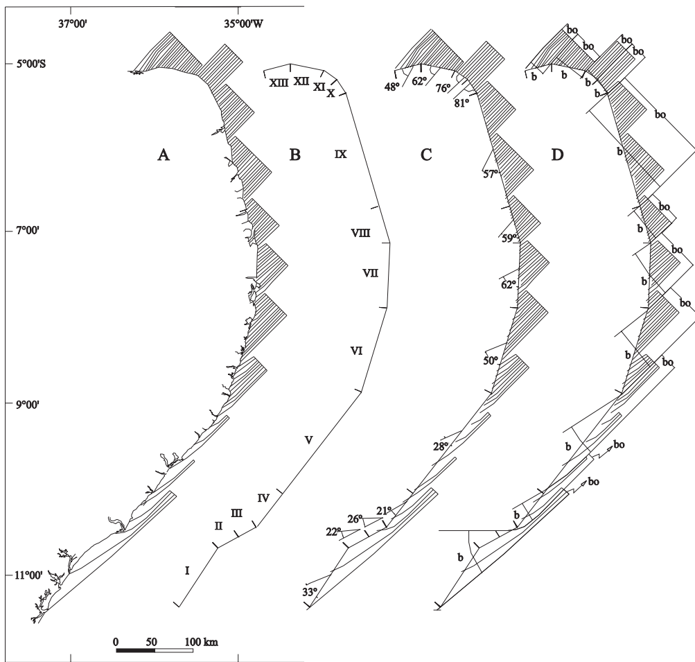
Fig. 2 – A – Refraction diagram for waves with a 5 sec period, arising from the NE (N45°). B – Different segments in which the coastline has been rectilinearized. C – Incidence angles formed by waves from NE in relation to the rectilinearized coastal segments. D – Measurements of b and b_0 for estimating the height of waves along the rectilinearized coastal segments.
