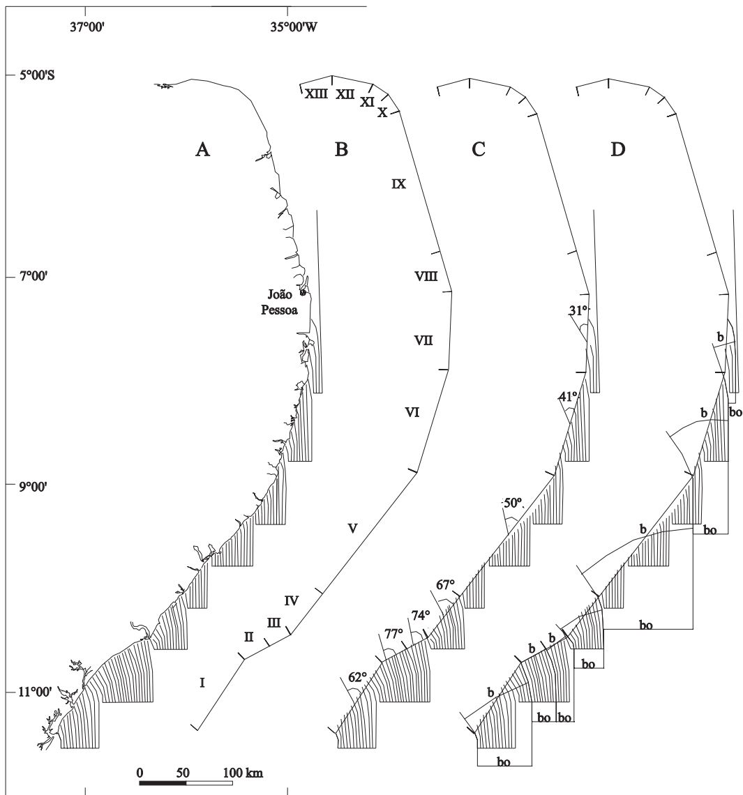
Fig. 5 – A – Refraction diagram for waves with a 6.5 sec period, arising from the S ( N180^\circ ). B – Different segments in which the coastline has been rectilinearized. C – Incidence angles formed by waves from S in relation to the rectilinearized coastal segments. D – Measurements of b and b_0 for estimating the height of waves along the rectilinearized coastal segments.
