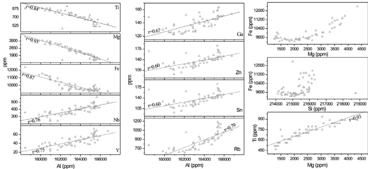
Fig. 4 – Selected bivariate diagrams showing the trend compositional of the muscovite megacrystal studied. Solid line is the best linear fit to the experimental data (n=56).
