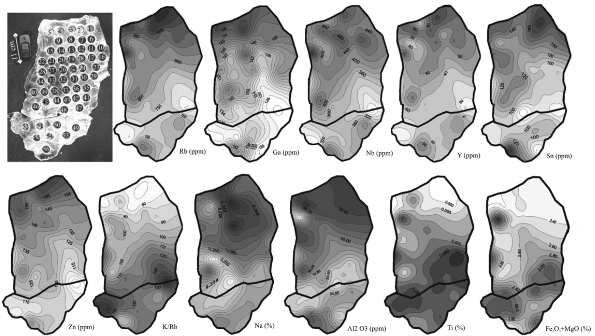
Fig. 3 – Sketch of studied muscovite plate with location of the analyzed points and distribution maps of the compositional contour lines for selected elements.
