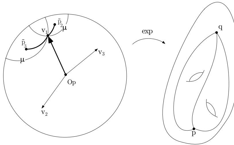
Fig. 1 – Mediatrices \mu corresponding to the focal decomposition. The \bar{d} -distance from v_1 to O_p, \bar{p}_2, \bar{p}_3 is \ell . The vectors v_1, v_2, v_3 have common exponential image q , while O_p, \bar{p}_2, \bar{p}_3 have exponential image p .
