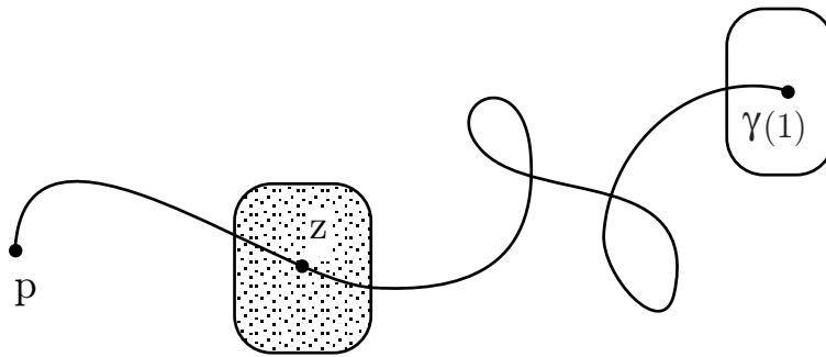
Fig. 2 – Varying g at a free spot z controls the endpoint q = \gamma(1) of the geodesic \gamma .
