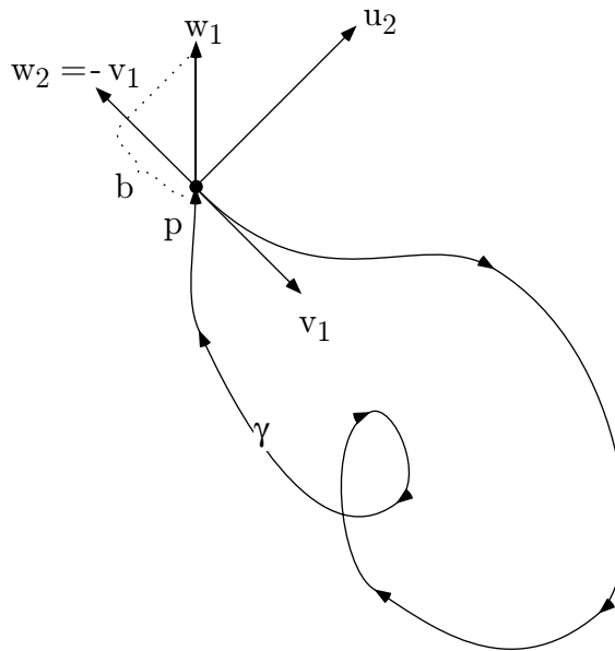
Fig. 3 – A geodesic loop.
