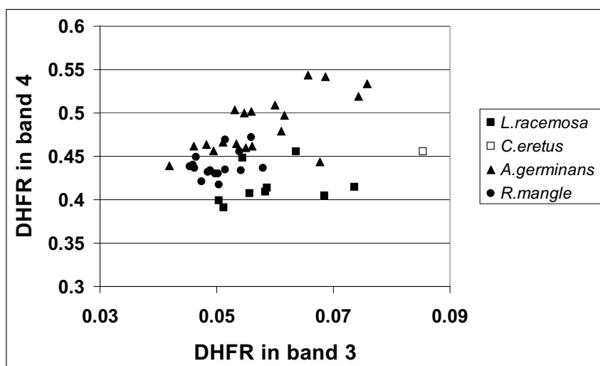
Fig. 4 – DHFR band 4 × DHFR band 3 scatter plot.
