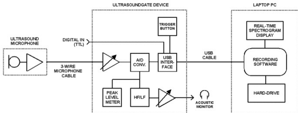
Fig. 2 – Principle of the UltraSoundGate system.
