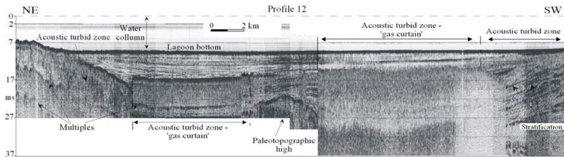
Fig. 3 – Linkage of gas occurrences to areas of paleotopographic lows in profile 12 (see Fig. 1 for location). Depths to water surface in two-way travelttime, in milliseconds (ms).
