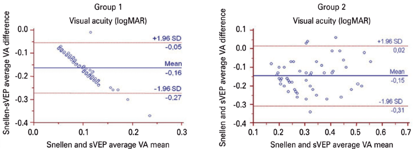
Figure 3. The Bland-Altman plot average difference was -0.16 logMAR in Group 1 and -0.15 logMAR in Group 2. The distribution of the differences between the Snellen best corrected visual acuity and mean sweep visual evoked potential visual acuity was \pm 0.11 logMAR in Group 1 and \pm 0.16 logMAR in Group 2. The 95% confidence intervals are represented by the dotted lines ( \pm 1.96 ).
