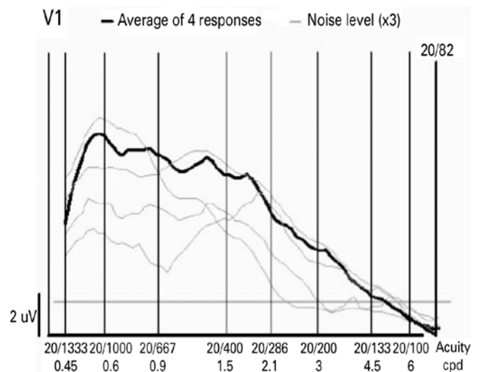
Figure 2. This graph shows the vector average of the different sweep responses recorded during the exam. From this vector average, the program automatically determines the visual acuity as the smallest pattern size that produces a response (20/82 in the present example).
