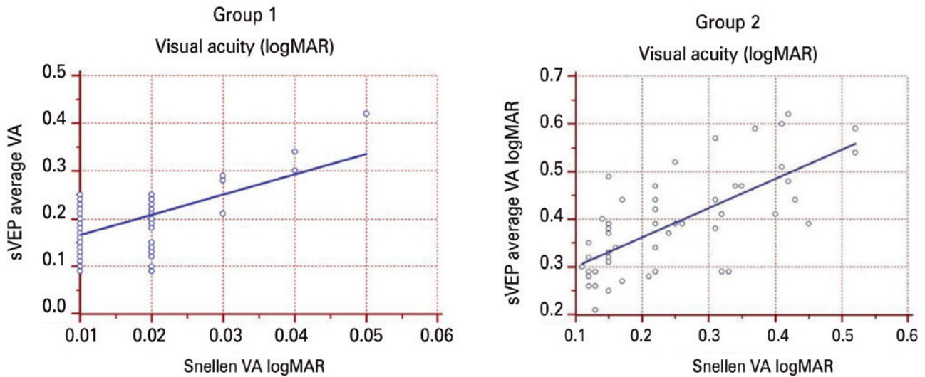
Figure 5. In Group 1, for the Snellen best corrected visual acuity and mean sweep visual evoked potential visual acuity, the regression equation was y = 0.12 + 4.3x , and the coefficient of determination ( R^2 ) was 0.30. In Group 2, the regression equation was y = 0.24 + 0.61x , and the R^2 was 0.50.
