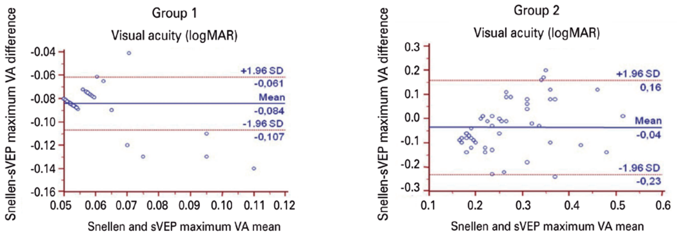
Figure 4. The Bland-Altman plot average difference was -0.08 logMAR in Group 1 and -0.04 logMAR in Group 2. The distribution of the differences between the Snellen best corrected visual acuity and mean sweep visual evoked potential visual acuity was \pm 0.023 logMAR in Group 1 and \pm 0.19 logMAR in Group 2. The 95% confidence intervals are represented by dotted lines ( \pm 1.96 ).
