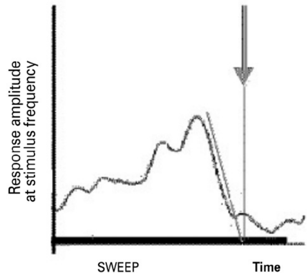
Figure 1. Each sweep is indicated by a vertical line, while its duration is indicated by a thick horizontal line. As the size of the pattern decreases, the amplitude of the response increases, reaches a maximum, then decreases rapidly. The sweep of the spatial resolution domain allows an estimation of visual acuity from the smallest pattern size producing a response.
