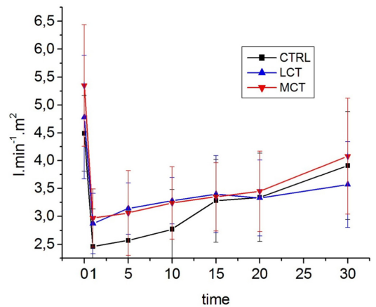
FIGURE 6 - Cardiac index.
