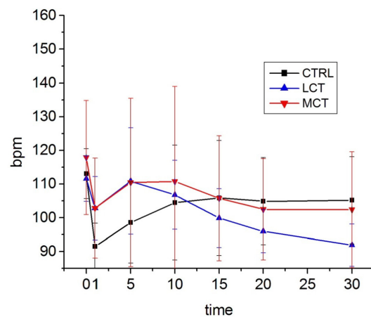
FIGURE 2 - Heart rate,
