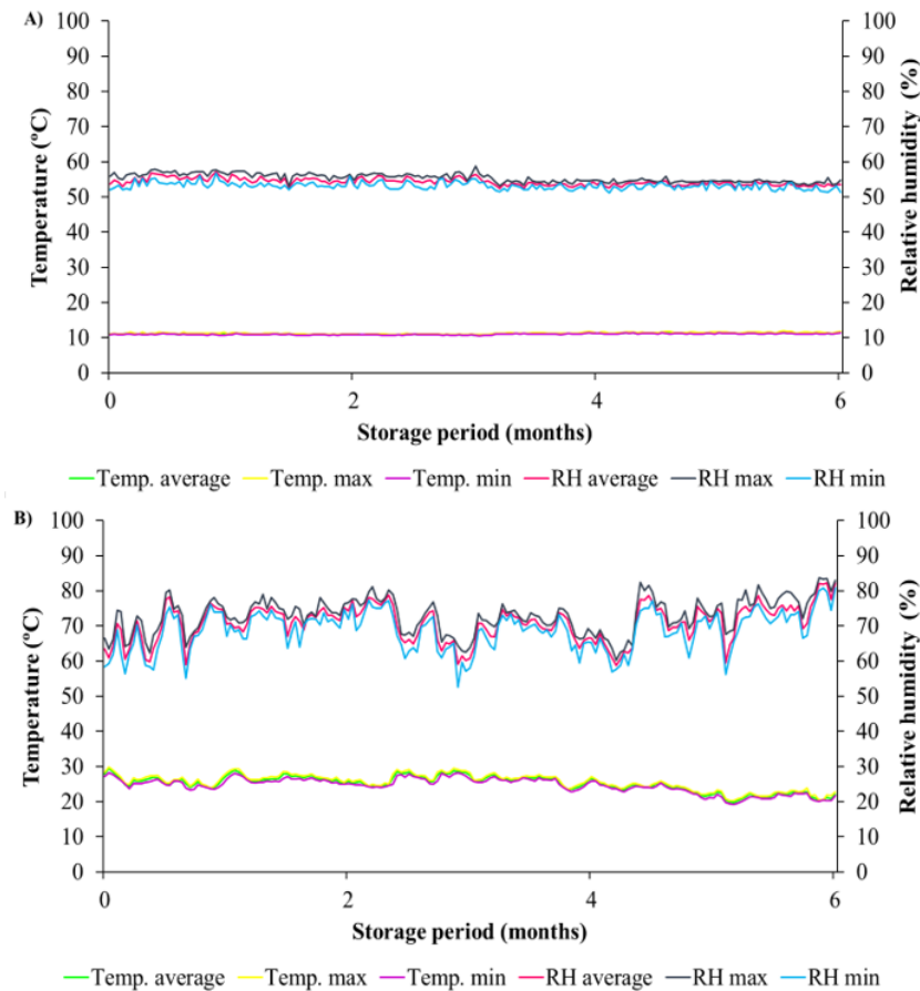
Figure 1. Maximum, average, and minimum daily temperature (°C) and maximum, average, and minimum daily relative humidity (RH) (%) during the storage period of soybean seeds in the cold and dry chamber (A) and uncontrolled environment (B).
