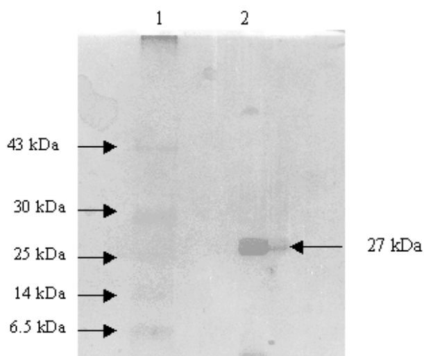
Figure 1. SDS-PAGE of final purification step of PE from potato. Lane 1 are Molecular weight markers (see Materials and Methods) and Lane 2 is potato PE.
