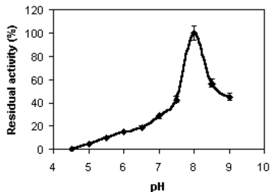
Figure 3. pH optimum determination of potato PE.
