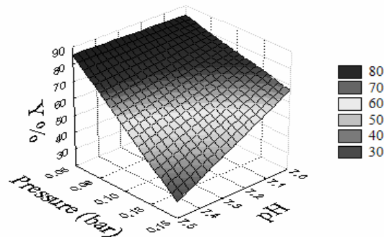
Figure 2 - RSM for describes to influence of the transmembrane pressure and pH on bromelain activity recovery (Y).
