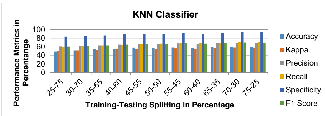
Figure 13. Performance evaluations of kNN classifier using data splitting method
