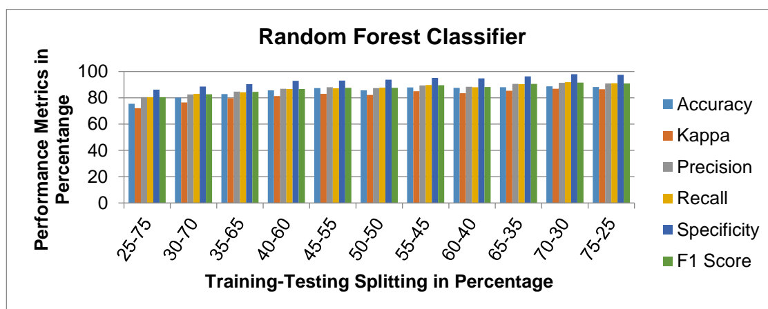
Figure 9. Performance evaluations of RF classifier using data splitting method
