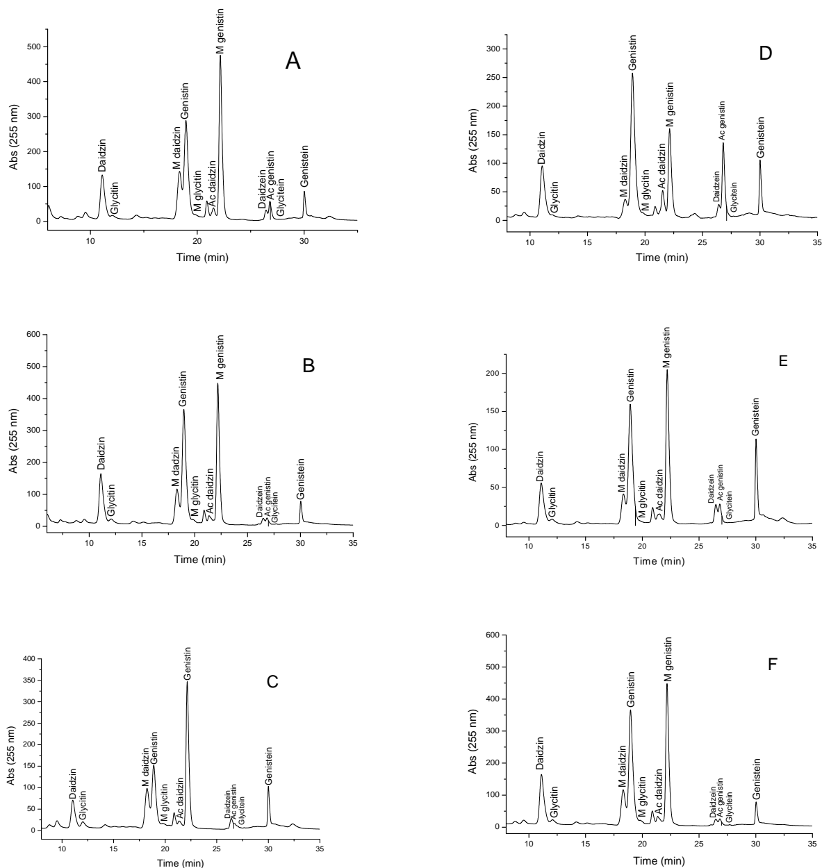
Figure 1 - HPLC chromatograms of isoflavones in (a) low fat soybean flour, (b) soy milk, (c) raw soybeans, (d) soy nuts, (e) Okara and (f) textured soy protein samples. The abbreviations M and Ac were used for malonyl and acetyl conjugates, respectively.
