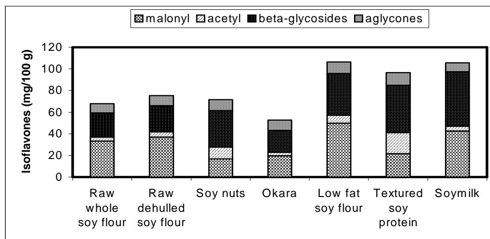
Figure 2 - Total isoflavone content and profile (naturally occurring aglycones, malonyl, acetyl, and \beta -glycosides derivatives) of Ecuadorian soy products.
