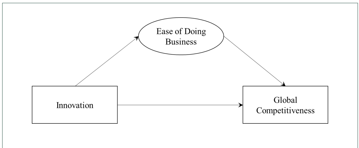
Figure 1. Theoretical model.
