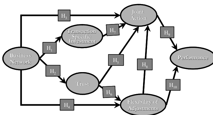
Figure 1: Theoretical Framework
