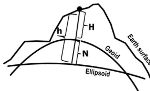
Figure 2: Geoidal height.
