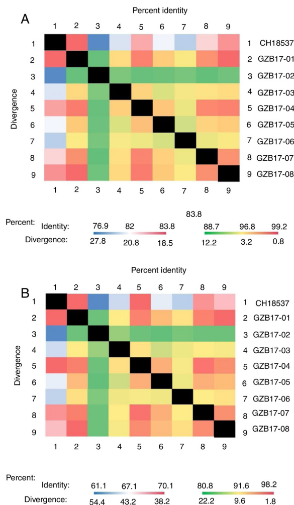
Fig. 3 – Comparison of homology between Guizhou HRSV subgroup B isolates 3' end of G gene nucleotide and amino acid sequences with that of the prototype strain CH18537 in colored heat map. A, comparison of nucleotide sequences homology of subgroup B; B, homology comparison of amino acid sequences of subgroup B. Red indicates the maximum identity, blue indicates the minimum identity, white indicates the middle value, green indicates the maximum divergence, red indicates the minimum divergence, yellow indicates the middle value.
