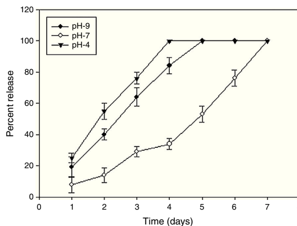
Fig. 2 – Percent release of AMB from fibrin microsphere. Fibrin microsphere containing entrapped AMB was incubated in different pH at 25 °C and release kinetics of the drug was determined spectrophotometrically. Each value represents mean ± SD of three determinations.
