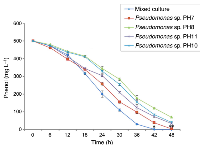
Fig. 2 – Degradation curve of phenol using pure and mixed cultures. Phenol (500 mg L -1 ) was added to the MM medium, inoculated with 2% (v/v) cultures and incubated at 30 °C and 200 rpm. Statistical analyses were performed with Student's t test in SPSS 17.0 software (SPSS Inc, Chicago, IL, USA), and the error bars represent the means (±SD) of three independent experiments. * The phenol degradation rate of the mixed culture is significantly higher than the rates for strains PH7, PH8, PH11, and PH10 ( p < 0.001 ). ** The phenol degradation rate of strain PH7 is significantly higher in comparison with strains PH8, PH11, and PH10 ( p < 0.001 ).
