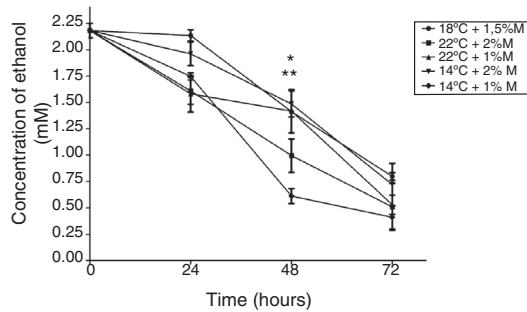
Fig. 5 – Ethanol concentration. Representative graphic of the ethanol concentration in different culture conditions. Each point represents the mean \pm SD ( n=3 ). Statistical analysis by two-way ANOVA–Bonferroni’s post-test. * p < 0.05 (22 °C + 2%M vs. all other conditions); ** p < 0.05 (14 °C + 1%M vs. all other conditions).
