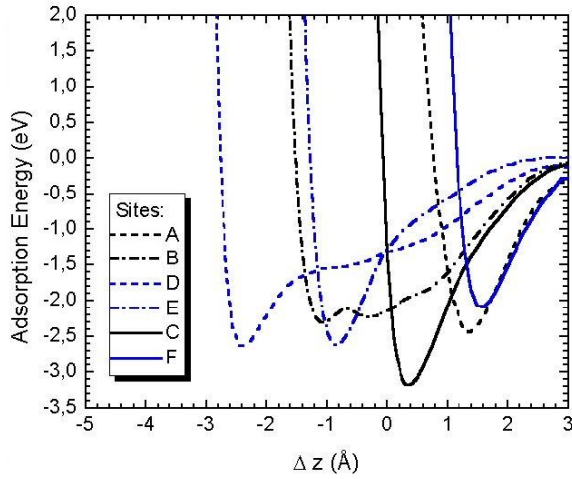
FIG. 2: Adsorption energy variation as a function of the distance of the adsorbed N atom from the As dimers, \Delta z (in Å), over the GaAs (100) (2×1) surface at the sites A, B, C, D, E and F, as defined in Fig. 1.
