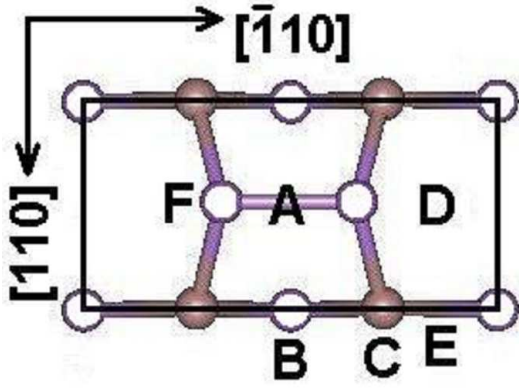
FIG. 1: Top view of the possible N adsorption sites over As-terminated GaAs (100) (2×1) surfaces. The open circles are the As atoms, while the full circles are the Ga ones.
