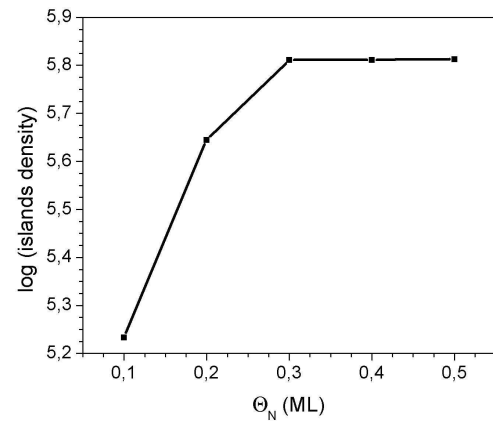
FIG. 6: Calculated variation of the logarithm of the islands density as a function of the N coverage (the growth temperature is 700 K).
