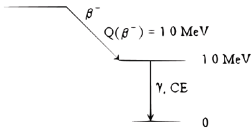
Figure 1. Decay scheme considered in the Monte Carlo simulation.
