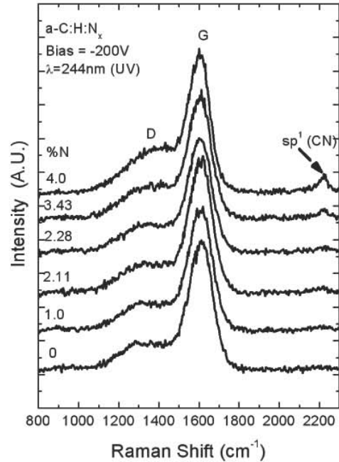
FIG. 2: UV Raman spectra from a-C:H:N_x (-200V) alloys.
