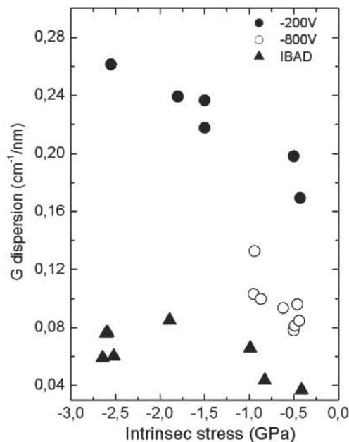
FIG. 5: G dispersion as a function of the intrinsic stress for a-C:H:N x (-200V), a-C:H:N x (-800V) and a-C:N x .
