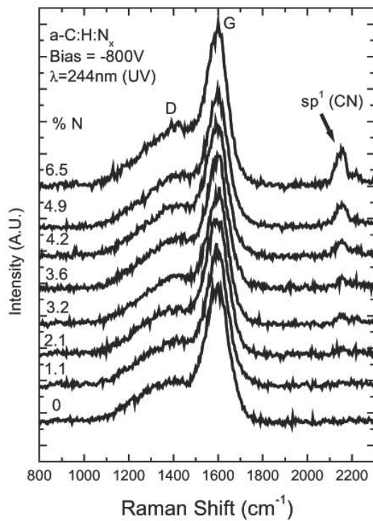
FIG. 1: UV Raman spectra from a-C:H:N_x (-800V) alloys.
