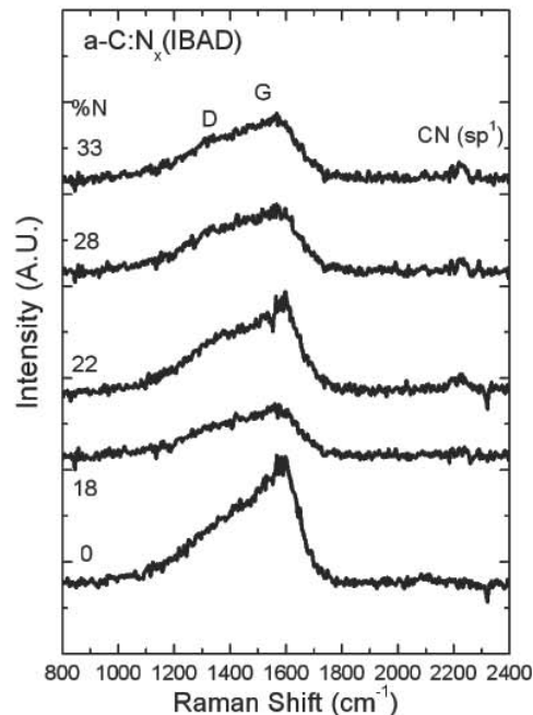
FIG. 3: UV Raman spectra from a-C:N_x films (IBAD).
