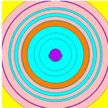
Figure 2. Frontal view of the beam holder with the sample port and Pb(1cm)-reflector.
