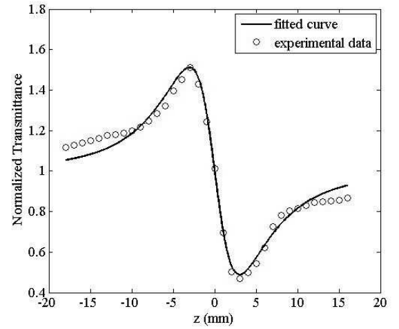
FIG. 6: Closed aperture Z-scan experimental curve for (Au-PVA) nano-fluid measured for sample with particle size of 10.5 nm.
