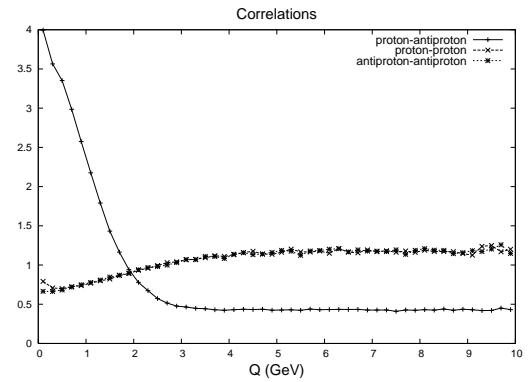
FIG. 4: MC results for the ratio C_{MC}(Q) = MC(Q)/MC_{\text{mix}}(Q) for pp - ( \times ) and p\bar{p} -pairs ( + ).
