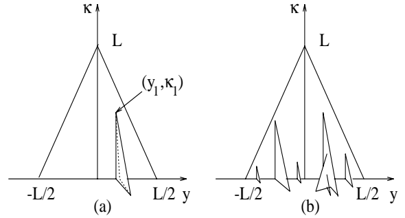
FIG. 1: The phase space for gluon emission in e^+e^- -ann. is a triangular region in the (y, \kappa = \ln k_{\perp}^2) -plane. The height of the triangle is given by L = \ln s . When one gluon is emitted at (y_1, \kappa_1) a second gluon with smaller k_{\perp} can be emitted in the larger phase space shown in Fig. (a). Further softer emissions give the fractal phase space in Fig. (b).
