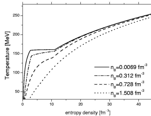
Figure 3. Temperature versus entropy density for various baryon densities.
