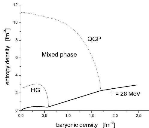
Figure 2. A phase diagram in (s, n_B) plane.
