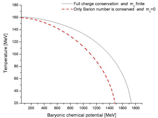
Figure 1. Phase diagrams for T and \mu_B .
