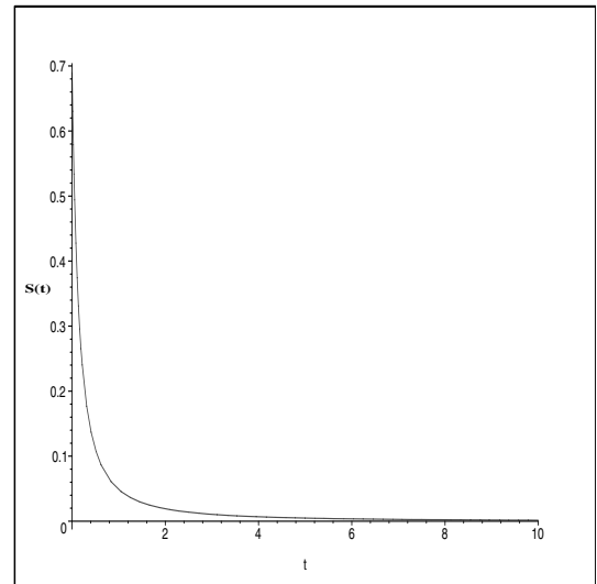
FIG. 2: The plot of scale factor R(t) vs time with parameters \alpha_1 = 1.00, \alpha_2 = 4.00, \alpha_3 = 1.00 and \gamma = 0.5
