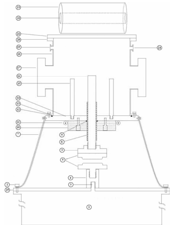
FIG. 2: The arrangement for SBUPF1 . 1= 25-kV,8.6- \mu\text{F} capacitor; 2 = capacitor Earth stud ; 3 = capacitor H.V electrode ; 4 = connector ; 5 = parallel plate spark gap (indicated with details in fig. 1) ; 6 = connector ; 7 = copper strap ; 8 = pyrex insulator sleeve ; 9 = O-ring seal ; 10 = polyethylene for holding the O-ring ; 11 = Rogowski coil ; 12 = steel flange ; 13 = O-ring seal ; 14 = cathode collector plate ; 15 = focus cathode (12 rods) ; 16 = focus anode ; 17 = chamber window ; 18 = focus chamber ; 19 = outlet to vacuum pump ; 20 = flange ; 21 = back flange ; 22 = the hole for setting detector and foil ; 23 = polyethylene for thermalizing the neutron ; 24 = inlet for test gas ; 25 = insulator cap of capacitor.
