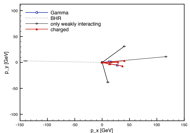
FIG. 1: Transverse momentum distribution of a single BH event at the LHC with an initial energy of 2 TeV and a BHR mass of 1 TeV and p_T > 10 GeV. The dashed line represents the BHR transverse momentum which, in the case of a neutral BHR, would be not visible in the detector [37].
