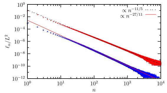
FIG. 7: Distribution normalized to the volume L^2 of the hulls and external perimeters of FK clusters in the 2D Ising model at criticality on a square lattice of linear size L = 512 . Statistical error bars are omitted from the data points for clarity. The straight lines are one-parameter fits through the data points with the slopes fixed to the expected values. For clarity, the external perimeters distribution is shifted downward by two decades.
