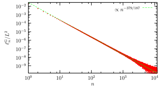
FIG. 5: Distribution \ell_n^G normalized to the volume L^2 of geometrical clusters in the 2D Ising model at criticality on a square lattice of linear size L = 512 . Statistical error bars are omitted from the data points for clarity. The straight line is a one-parameter fit through the data points with (minus) the slope fixed to the value \tau^G = 379/187 = 2.02673\dots . The fit illustrates that asymptotically the distribution is algebraic at criticality.
