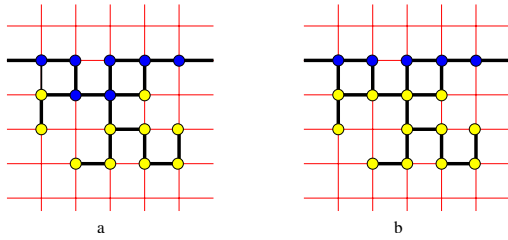
FIG. 6: In both panels, a piece of the same single FK cluster of nearest neighbor sites (filled circles) connected by bonds (black links) is shown. Two different external boundaries can be defined: (a) The hull (dark filled circles) is found by allowing a random walker tracing out the boundary to move only over set bonds. (b) The external perimeter (dark filled circles) is found by allowing the random walker to move to a nearest neighbor on the cluster boundary irrespective of whether the connecting bond is set or not. The external perimeter, which contains two sites less than the hull for this boundary segment, is therefore a smoother version of the hull.
