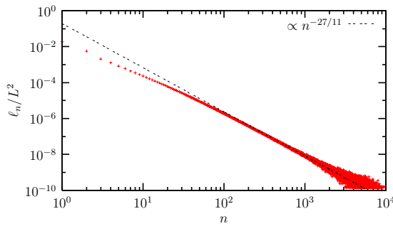
FIG. 8: Distribution normalized to the volume L^2 of the hulls of geometrical clusters in the 2D Ising model at criticality on a square lattice of linear size L = 512 . Statistical error bars are omitted from the data points for clarity. The straight line is a one-parameter fit through the data points with the slope fixed to the expected value.
