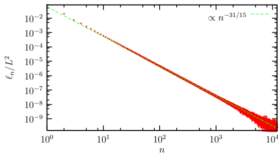
FIG. 3: Distribution \ell_n normalized to the volume L^2 of FK clusters in the 2D Ising model at criticality on a square lattice of linear size L = 512 . Statistical error bars are omitted from the data points for clarity. The straight line is a one-parameter fit through the data points with (minus) the slope fixed to the predicted value \tau = 31/15 = 2.06666\dots . The fit illustrates that asymptotically the distribution is algebraic, as expected at criticality.
