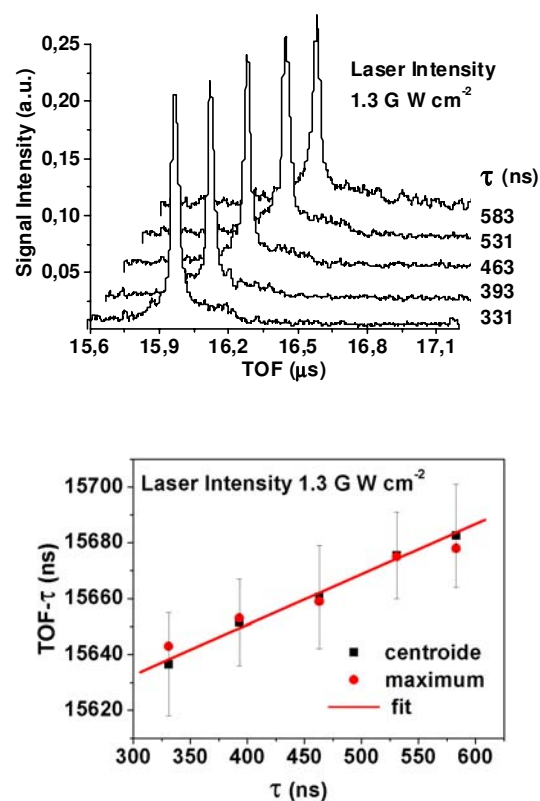
Figure 2. (a) The experimental spectra of the insulin ion (\text{M}+\text{H})^+ for the case of 1.3 \text{ G W cm}^{-2} laser intensity. (b) The maximum and the centroid evolution of the TOF peak for different applied delayed extraction time, \tau .
