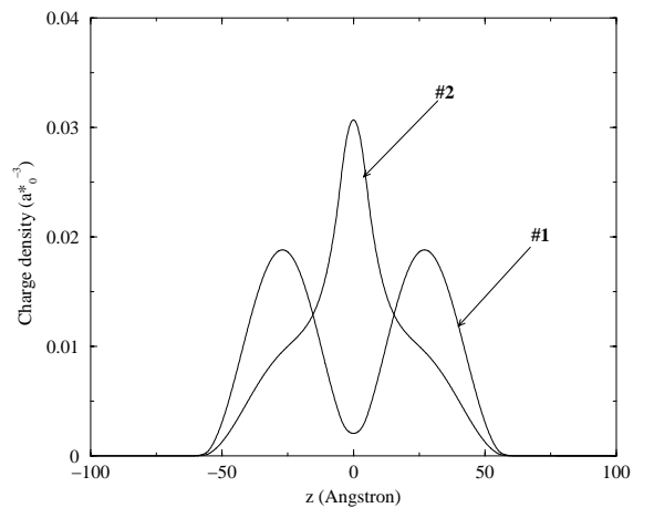
Figure 1. Charge density as a function of the distance to the center of the well. Sample #1: two GaAs quantum wells of 50Å separated by a 10Å barrier of \text{Ga}_{0.65-x}\text{Al}_{0.35}\text{Mn}_x . Sample #2: a 10Å \text{Ga}_{1-x}\text{Mn}_x\text{As} instead of the middle barrier.
