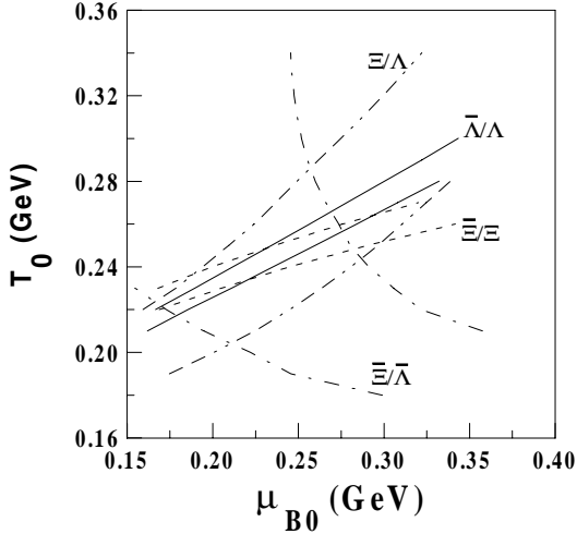
Figure 12. Window in initial conditions reproducing WA97 data in the case of an equation of state without excluded volume corrections. With volume corrections, the window is lower [17].
