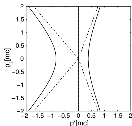
Figure 3. The solution to the equation d\sigma_\mu p^\mu = 0 for v = 0.65, 0 and -0.35 is given by the left hyperbola, the vertical axis and right hyperbola respectively. The permitted region is localized to the right of the curve in each of these three cases. The dashed lines correspond to the case of massless particles.
