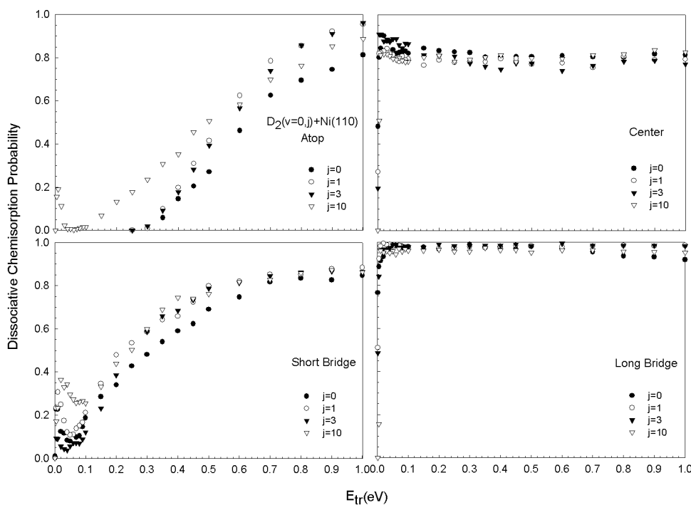
FIG. 1: The DC probabilities on the low index Ni(110) surface at the topologically different impact sites as a function of the translational energy for the D_2(v, j) molecule for various initial rotational states, j = 0, 1, 3 and 10 at v = 0 .
