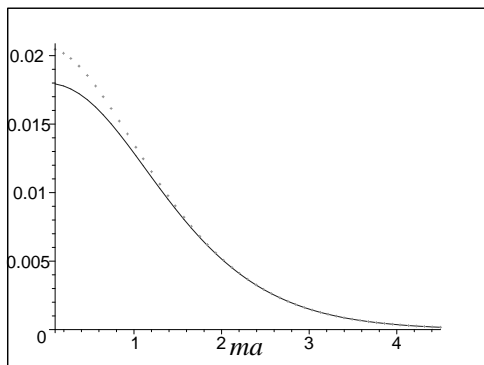
Figure 5. In this graphic we plot the modules of pressures with mixed BC (line) and Dirichlet BC (point).
