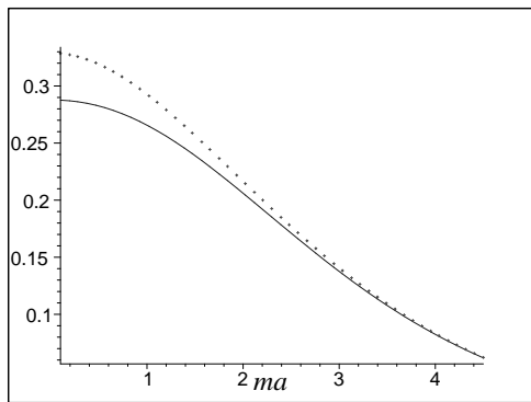
Figure 4. In this graphic: we plot the modules of pressures with antiperiodic BC (line) and periodic BC (point).
