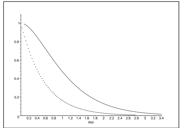
Figure 3. From top to bottom we have the Casimir energies for a massive bosonic field subjected to Dirichlet BC and for a massive fermionic field submitted to MIT BC, respectively.
