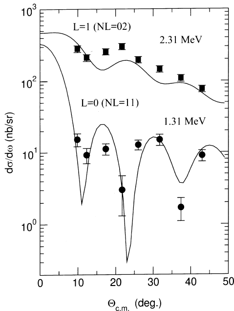
Figure 2. Angular distributions for the ^{14}\text{N}(^3\text{He},^6\text{He})^{11}\text{N} reaction for the transitions denoted. The curves are the results of DWBA calculations with the transferred angular momenta ( L ) indicated.
