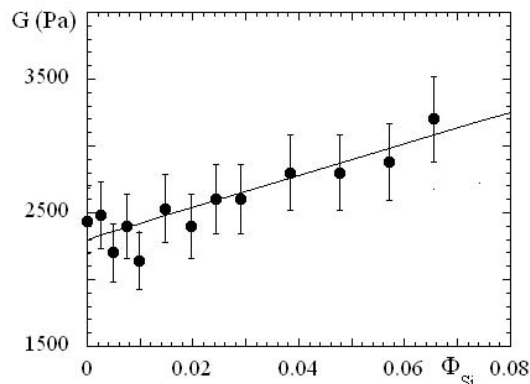
FIG. 4: Modulus G in Pa of filled 35k copolymer network ( \Phi_p = 3\% ) for increasing silica volume fraction \Phi_{Si} . All samples are at pH 10.
