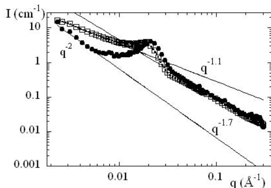
FIG. 8: Scattered intensity I in \text{cm}^{-1} as a function of wave vector q in \text{\AA}^{-1} in pure D_2O of 35k copolymer network with a volume fraction \Phi_p = 2\% ( \square ). The data is compared to the intensity of the same network containing 6.54%V of index matched silica particles ( \bullet , \rho_{\text{solv}} = \rho_{\text{Si}} = 3.5 \cdot 10^{10} \text{cm}^{-2} ). The latter intensity has been rescaled to the one of the pure copolymer in order to compensate the differences in contrast.
