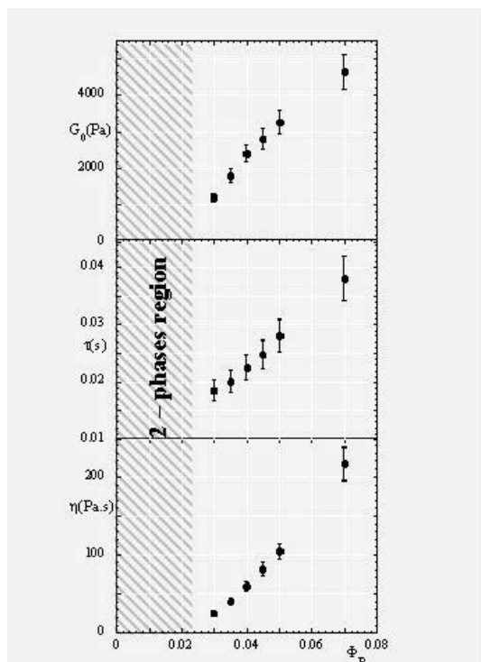
FIG. 3: Modulus G in Pa , \tau in s and \eta in Pa\cdot s of 35k copolymer network as a function of polymer volume fraction \Phi_p .
