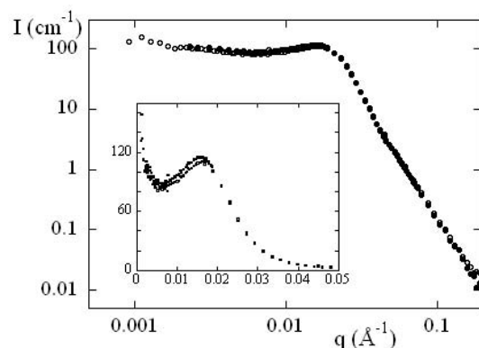
FIG. 9: Scattered intensity I in \text{cm}^{-1} as a function of wave vector q in \text{\AA}^{-1} of filled 35k networks containing contrast-matched microemulsion ( \circ , \Phi_{\text{Si}} = 6\% , R = 30 \text{\AA} , 4%, \rho_{\text{solv}} = \rho_m = 0.3 \cdot 10^{10} \text{cm}^{-2} ). This is compared to the intensity of pure silica ( \bullet ) at the same volume fraction, rescaled to identical contrast conditions.
