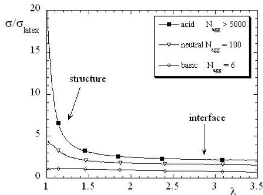
FIG. 1: Reinforcement factor of silica-latex nanocomposites ( \Phi_{si} = 5\% , three samples at pH ca. 4, 7 and 9), as a function of relative elongation \lambda = L/L_0 . The average aggregation numbers have been measured by Small Angle Neutron Scattering, see text for details.
