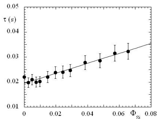
FIG. 5: Relaxation time in s of filled 35k copolymer network ( \Phi_p = 3\% ) for increasing silica volume fraction \Phi_{Si} . All samples are at pH 10.
