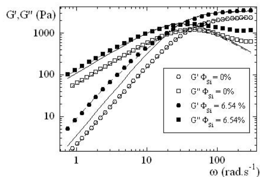
FIG. 7: Storage G' (Pa) (●) and loss G'' (Pa) (■) modulus as a function of \omega of (a) a filled 35k copolymer network ( \Phi_p = 3\% , \Phi_{Si} = 6.54\% ) compared with a copolymer network without silica ( G' (○) and G'' (□), \Phi_p = 3\% and \Phi_{Si} = 0\% ). With silica, departures from Maxwellian behaviour are emphasized in G'' at high \omega , and in G' at low \omega , which is illustrated by the solid line calculated for G' with silica, using a single relaxation time ( G_1 = 3200 Pa; \tau_1 = 0.032 s). The dotted lines are fits with a double Maxwell model G_1 = 3200 Pa; G_2 = 140 Pa, \tau_1 = 0.032 s; \tau_2 = 0.2 s for the filled network and G_1 = 2400 Pa; G_2 = 15 Pa; \tau_1 = 0.024 s; \tau_2 = 0.2 s for the pure network.
