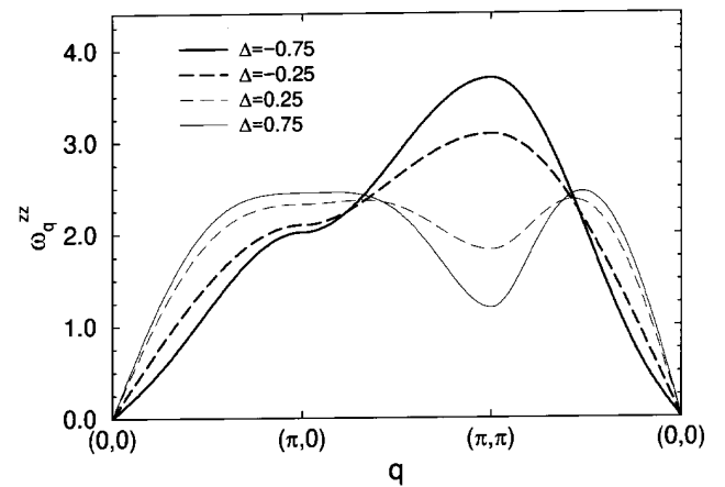
Figure 6. Longitudinal spin-wave dispersion \omega_{\mathbf{q}}^{zz} along the major symmetry directions of the 2D Brillouin zone.
