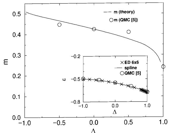
Figure 1. Magnetization m and ground-state energy \varepsilon of the 2D easy-plane XXZ model.
