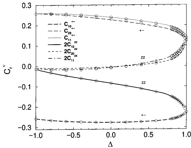
Figure 2. Transverse and longitudinal spin correlation functions C_{\mathbf{r}}^{\nu} at T = 0 . Symbols denote ED results obtained for a 6 \times 6 lattice.
