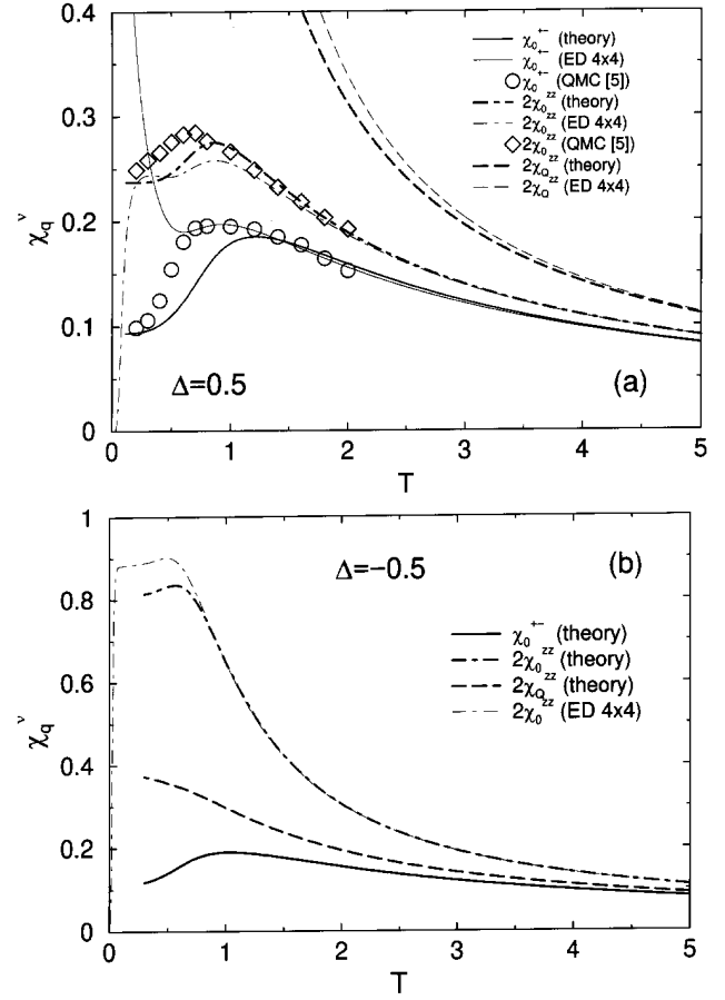
Figure 5. Longitudinal and transverse static spin susceptibilities \chi_{\mathbf{q}}^{\nu} as functions of temperature T for the 2D AFM (a) and FM (b) easy-plane XXZ models.
