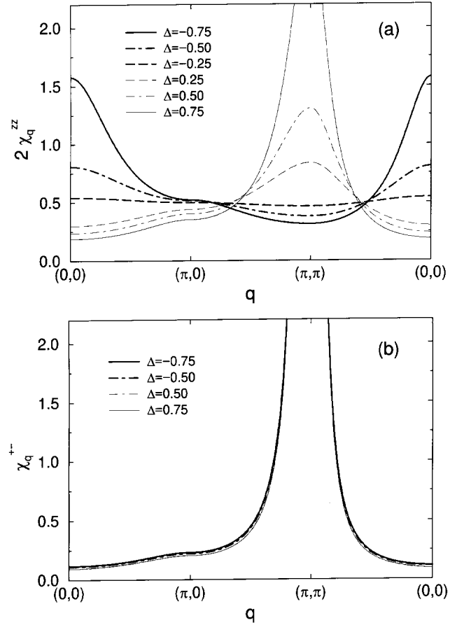
Figure 3. Wave-vector dependence of the longitudinal (a) and transverse (b) static susceptibilities \chi_{\mathbf{q}}^{\nu} at T = 0 .
