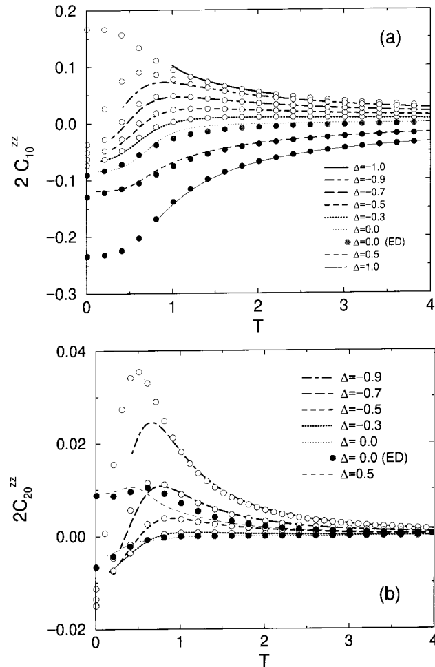
Figure 4. Temperature dependence of the NN (a) and next NN (b) longitudinal spin correlation functions C_{\mathbf{R}^{zz}} . Symbols denote ED results obtained for a 4x4 lattice.
