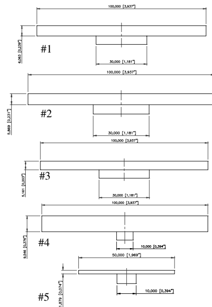
FIG. 1: The impedance matchers.
