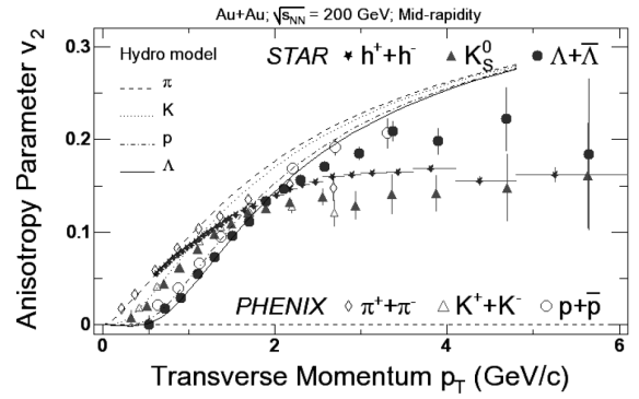
FIG. 5: Elliptic flow at RHIC energies as function of transverse momentum, compared to the simple ideal fluid hydrodynamical calculation. Figure adapted from the presentation of M. Gyulassy at International Symposium on Heavy Ion Collisions, Frankfurt, April, 2006.
