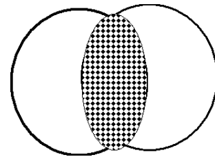
FIG. 2: Non central collision of two nuclei creates an anisotropic distribution of hot and dense matter which expands hydrodynamically.
