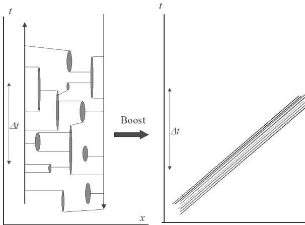
FIG. 1: Many virtual quarks and gluons form dressed valence particles in a hadron (left). These virtual particles behaves as real particles in a short time and distances (right).
