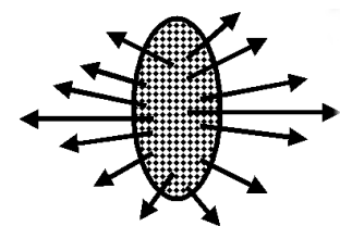
FIG. 3: Due to the sharp pressure gradient, the final state particles attain the anisotropic momentum distribution.
