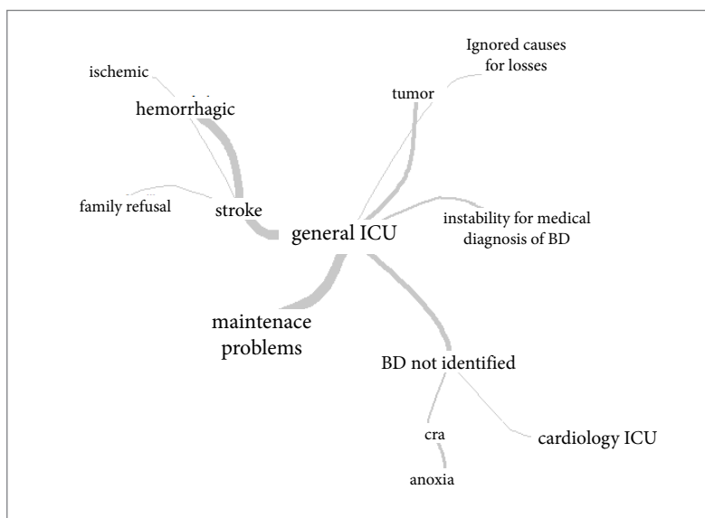
Figure 2. Textual similarity diagram considering the origin and cause of the escape of 35 patients.
