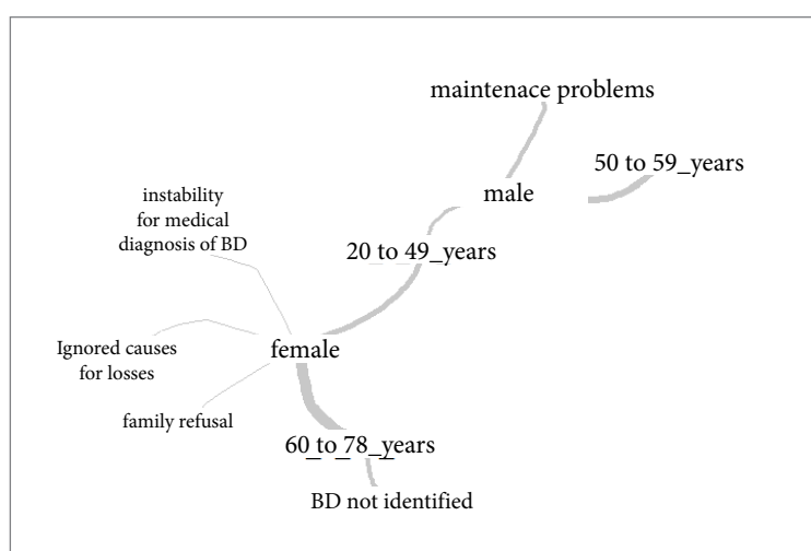
Figure 1. Textual similarity diagram considering the gender, age group and cause of escape of 35 patients.
